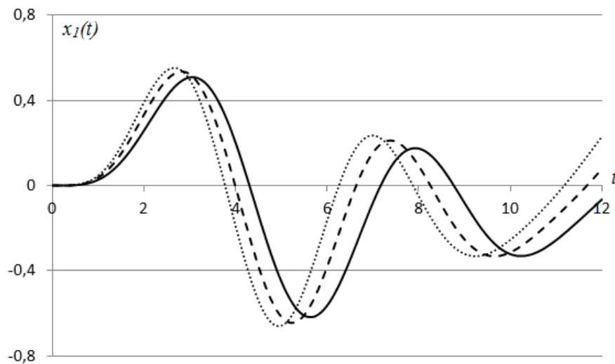
Figure 6. The influence of nonlinear properties of suspension on the mode of vibration of load of mass m_1
