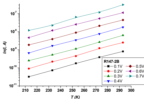
Figure 3. Temperature dependence of the forward current of the p-Sb 2 Se 3 /n-CdS heterostructure at various biases of 0.1–0.7 V
