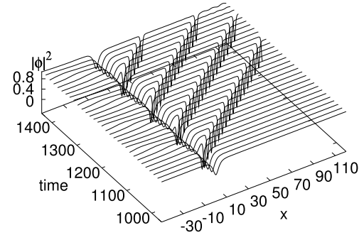
Fig. 4. Time evolution of a BEC flow in the transcritical regime when the NL barrier velocity v = 0.47 ( v_- < v < v_+ ). The NL barrier is taken in the form of V_m / \cosh(x/2) with V_m = 0.5 . During the time period from t = 0 to t = 1000 (that is not presented in the figure) the value of V_m is adiabatically being increased from 0 to 0.5. Further evolution is given at V_m = 0.5 .
