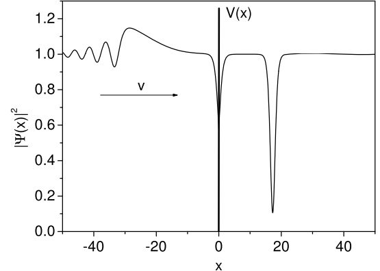
Fig. 7. The BEC density profile of a decaying unstable steady state at t = 180 . The flow velocity v and strength of the barrier \gamma are the same as in Fig. 6.
