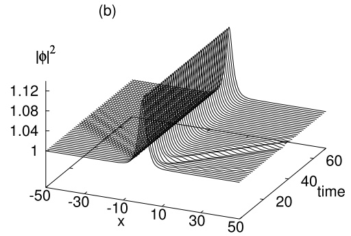
Fig. 3. Time evolution of a BEC flow in (a) subcritical regime, v = 0.373 and (b) supercritical regime, v = 2.517 through a nonlinear repulsive potential barrier V_m / \cosh(x/2) with V_m = 0.5 . The initial wave packet and distribution of the BEC local velocities u(x) are taken in the form determined by formulas (16), (17) and Eq. (10).
