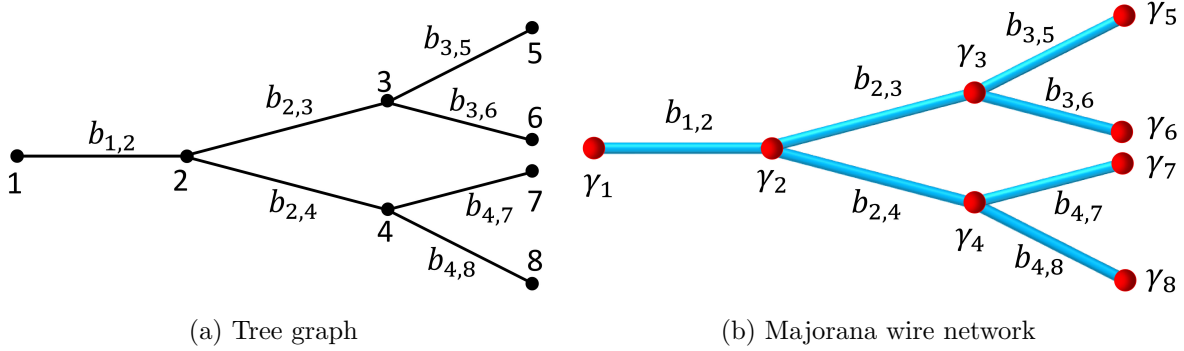
Figure 1: Tree graph based Majorana wire network
