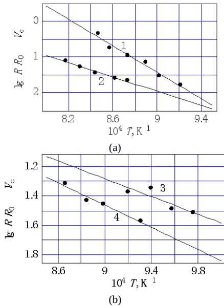
Figure 3. R(T_f) for DSG mentioned above (see Introduction). Solid lines are fitting of (5) to experimental data by the least squares method.
