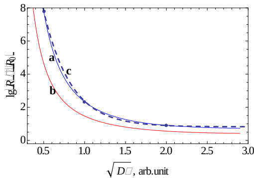
Figure 7. The result of simulation R(\tau) of DSG for r , \mu\text{m} : 0.5 (a); 1 (b). L \approx 5 \mu\text{m} . The function a + b \exp(-c\sqrt{\tau}) (dotted line) have been fitted to curve a in the 3 points.
