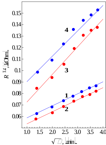
Figure 6. R(\tau) for DSG at T_f , K: 1073 (1, 2) and 1123 (3, 4). Temperature increasing rate is higher for data 1 and 2, than for data 3 and 4. Points are recalculated from [16] in accordance with (7). DSG composition isn't varied.
