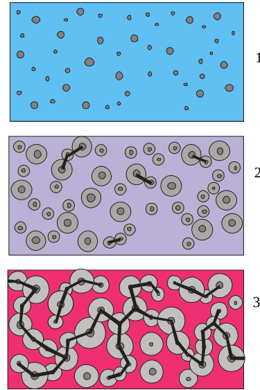
Figure 4. Generation of percolation levels due to diffusion (schematically). The bold curve is the infinite cluster. Gray circles represent diffusion zones. T_f in 3 is higher than in 1. \tau = \text{const} .
