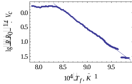
Figure 5. R(T_f) , recalculated data from [16] in accordance with (5). The solid line is fitting of (5) with R_0 = 10 Ohm, t = 1.7 , V_c = 0.16 .
