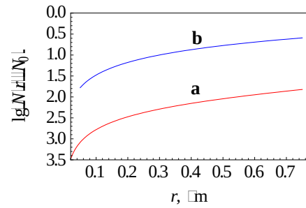
Figure 8. Effect of the main size of dopant particles on concentration of the dopant atoms at the point x = L/2 = 2.5 \mu\text{m} between the neighbor dopant particles (simulation, see Figures 2 and 7). Content of dopant in DSG is 2 times less for curve a than for curve b. The diffusion duration accords to the diffusion length \sqrt{D\tau} = 1.25 \mu\text{m} .
