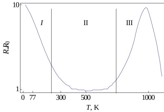
Figure 1. Resistivity vs temperature for DSG (schematically). Regions I, II and III correspond to low, middle and high temperature.
